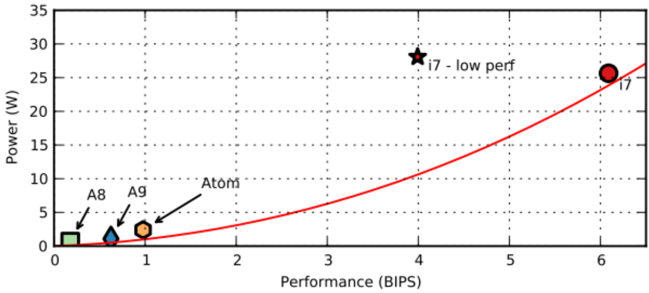
Figure 14. Power Performance Trade-offs.
