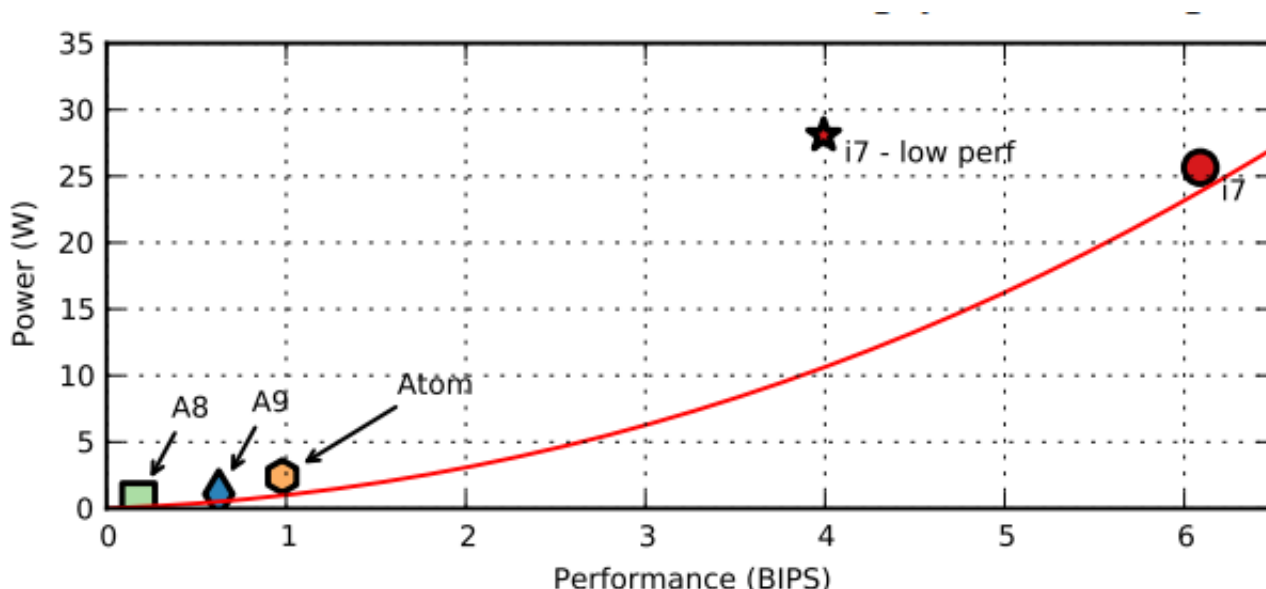
Figure 14. Power Performance Trade-offs.
